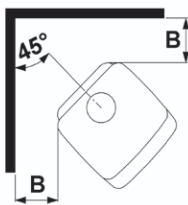
1410 corner installation 1440 corner installation
